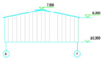
1 axis elevation
