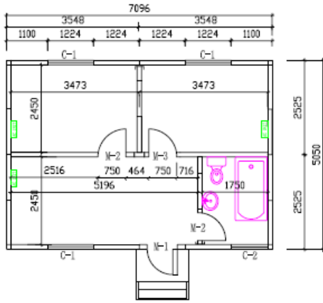
House plan
